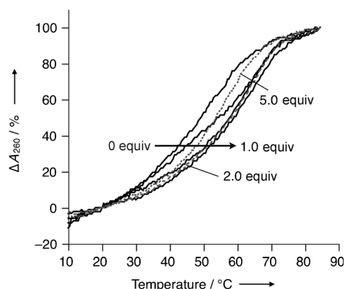
Figure 2. Melting curves of the bpy-modified DNA three-way junction ( L 1 L 2 L 3 ) in the presence of different concentrations of Ni II ions. [ L 1 L 2 L 3 ] = 1.0 μM, [Ni II ] = 0, 0.3, 0.7, 1.0 (—), 2.0 (----), and 5.0 μM (.....) in 10 mM MOPS buffer (pH 7.0), 100 mM NaCl, 0.2 °C min -1 , \Delta A_{260} = \{A_{260}(t^\circ\text{C}) - A_{260}(20^\circ\text{C})\} / \{A_{260}(85^\circ\text{C}) - A_{260}(20^\circ\text{C})\} \times 100 .
